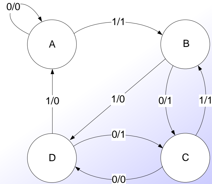
Mealy
