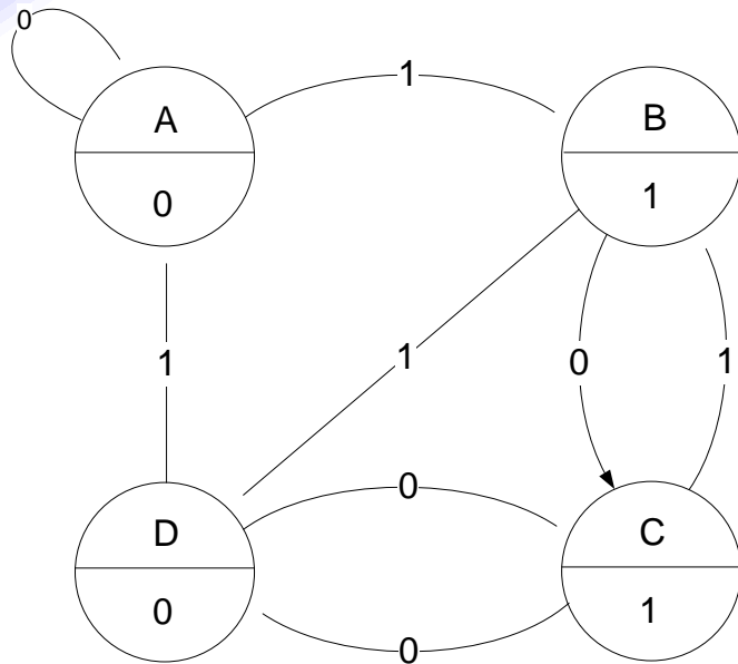
Moore
