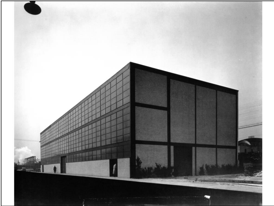
L. Mies van der Rohe, Minerals and Metals Research Center, Campus dell'Illinois Institute of Technology, 1941-43
