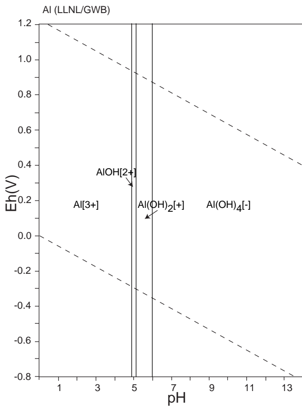
Figure 7: Eh-pH diagrams of the system Al-O-H (1). \Sigma \text{Al} = 10^{-10} , 298.15K, 10^5 Pa.
