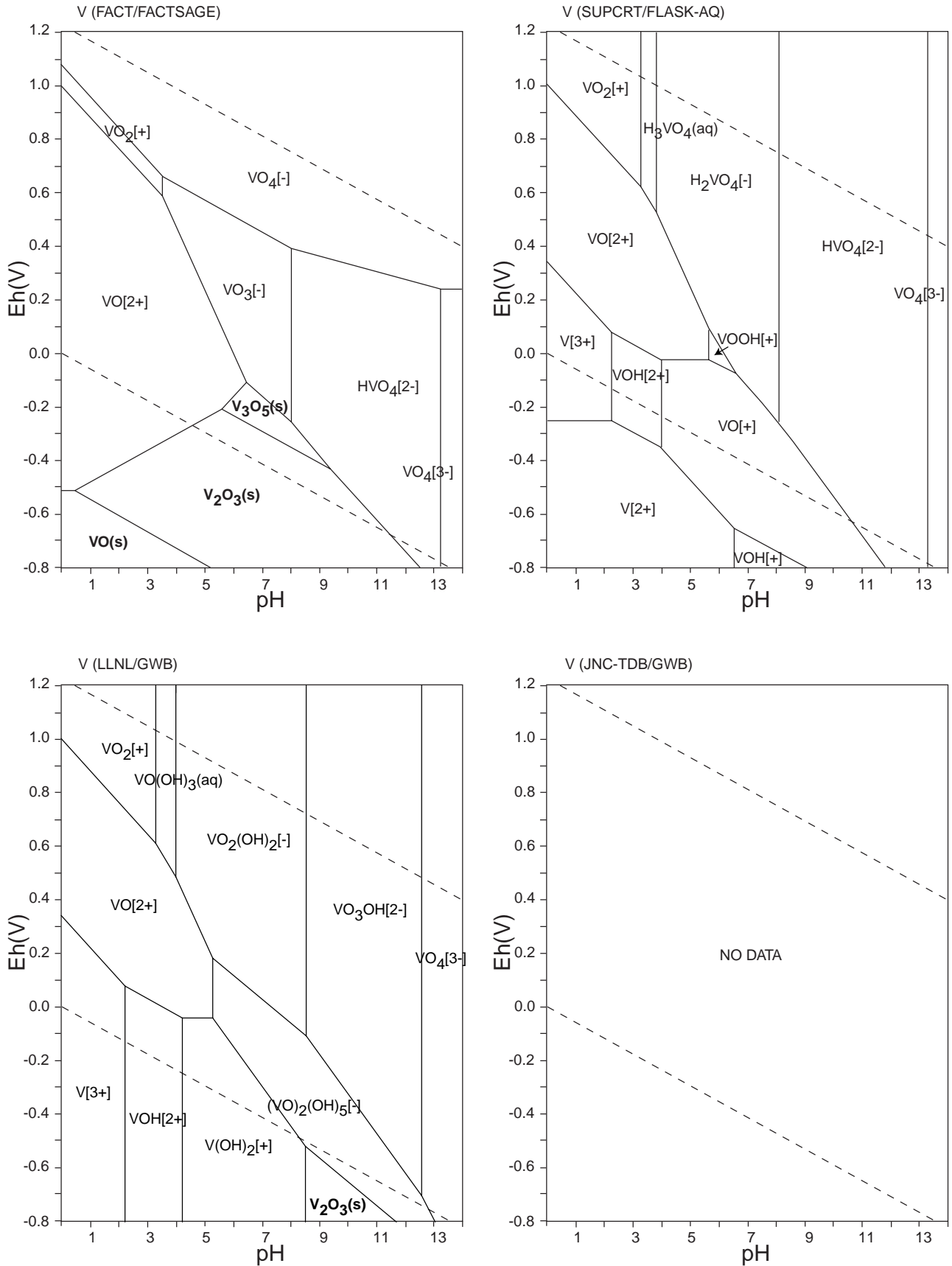
Figure 131: Eh-pH diagrams of the system V-O-H (1). \Sigma V = 10^{-10} , 298.15K, 10^5 Pa.
