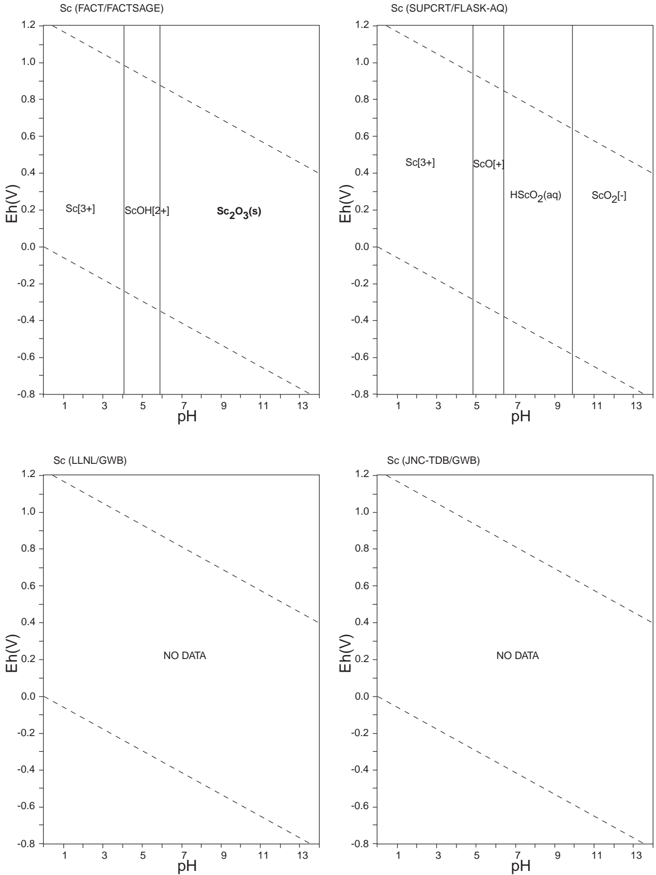
Figure 110: Eh-pH diagrams of the system Sc-O-H. \sum \text{Sc} = 10^{-10} , 298.15K, 10^5 Pa.
