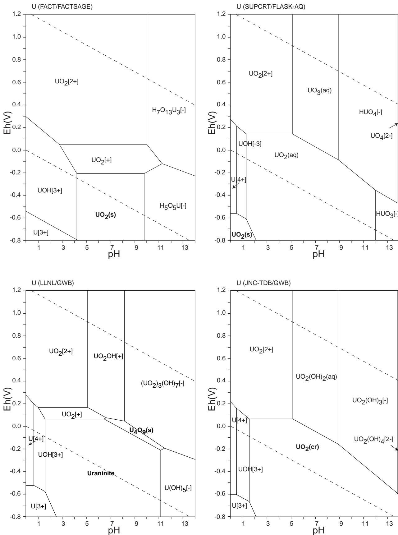
Figure 129: Eh-pH diagrams of the system U-O-H (1). \Sigma \text{U} = 10^{-10} , 298.15K, 10^5 Pa.
