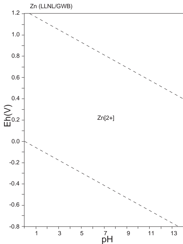
Figure 136: Eh-pH diagrams of the system Zn-O-H (1). \sum Zn = 10^{-10} , 298.15K, 10^5 Pa.
