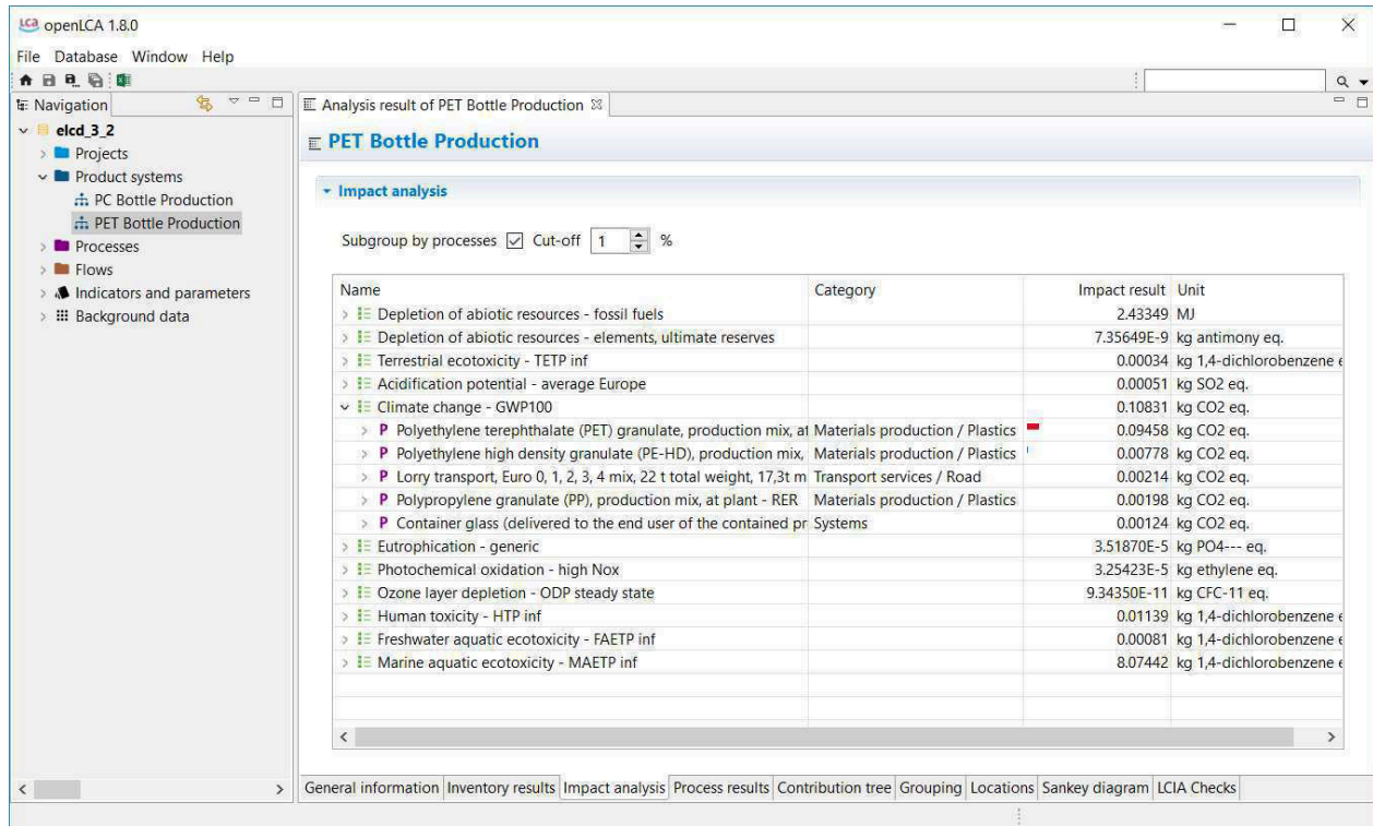
Figure 7.4: Impact analysis
