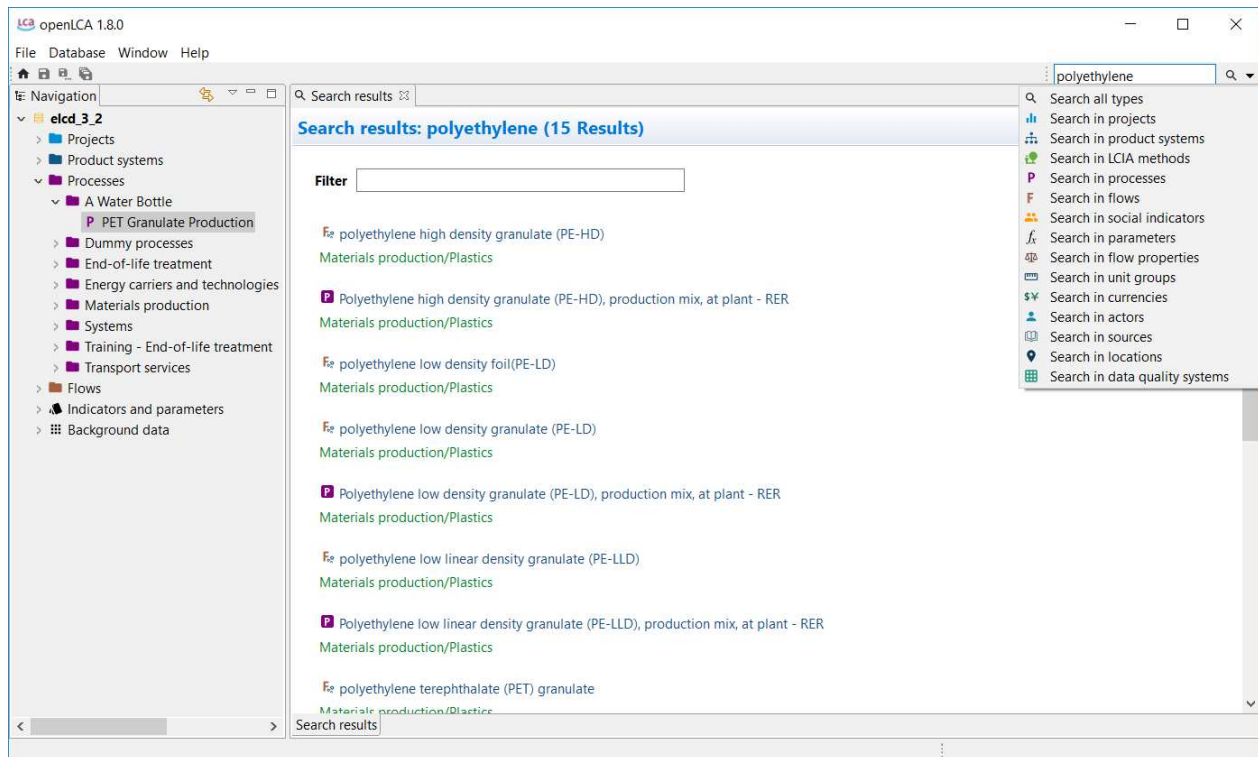
Figure 4.7: Search function
