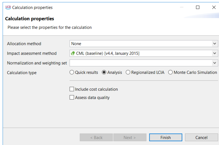
Figure 7.2: Calculation properties
