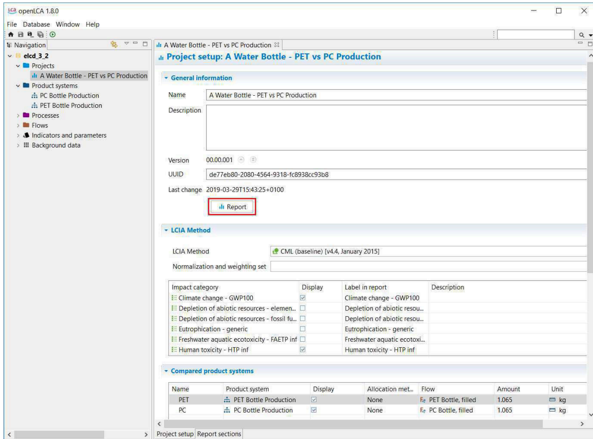
Figure 7.5: Project setup
