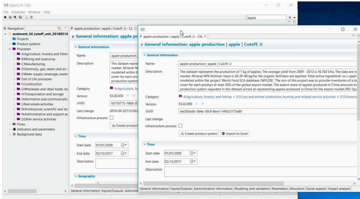
Figure 11.5: Detached windows
