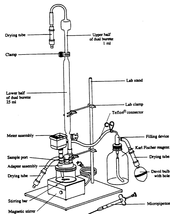
6-6 figure Karl Fischer titration unit. (Courtesy of Lab Industries, Inc., Berkeley, CA.)
