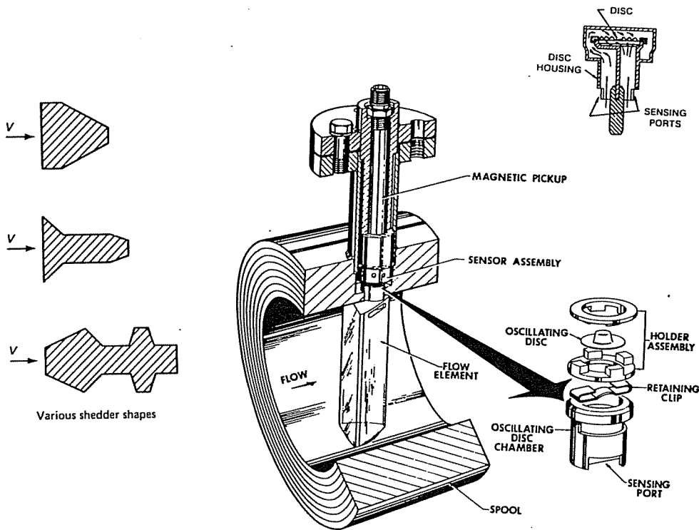
Figure 7.46 Vortex-shedding flowmeter details. (Courtesy Neptune Eastech)
