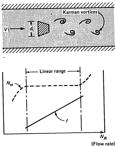
Figure 7.45 Vortex-shedding flowmeter principles.
