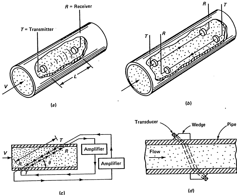
Figure 7.43 Ultrasonic flowmeters.
