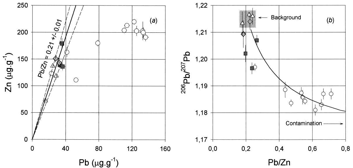
Fig. 4. (a) Pb vs. Zn diagram (both in \mu\text{g}\cdot\text{g}^{-1} ). (b) ^{206}\text{Pb}/^{207}\text{Pb} vs. Pb/Zn diagram. The hyperbolic curve is constructed from binary mixing between a background component ( \text{Pb/Zn} = 0.21 , ^{206}\text{Pb}/^{207}\text{Pb} = 1.215 ) and a contamination source characterised by a Pb/Zn ratio of 1 and ^{206}\text{Pb}/^{207}\text{Pb} ratio of 1.177. ( \Delta ) 3500–5000 years BP, ( \blacklozenge ) 3000–3500 years BP, ( \blacksquare ) 900–1500 years BP and ( \circ ) 500–900 years BP.
