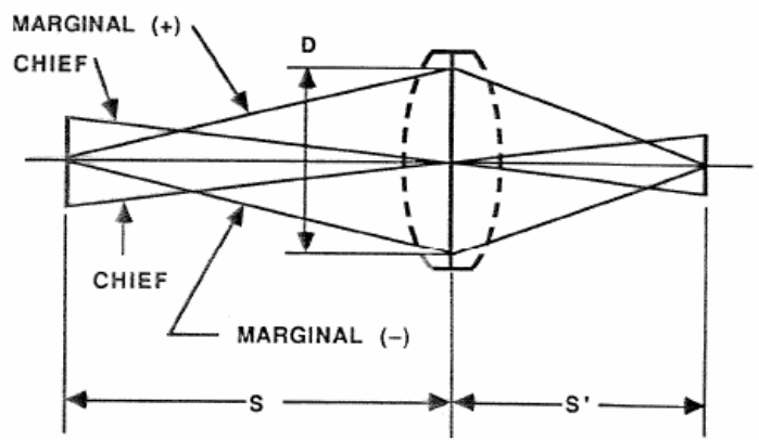
OBJECT AND IMAGE AT FINITE DISTANCES S'/D = (F/\#)_{\text{EFFECTIVE}}
